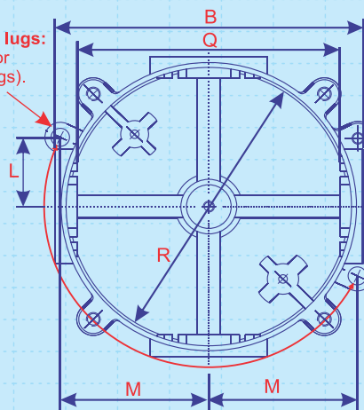
ZED® JUNCTION BOX DIMENSIONS - RIGHT ANGLE ENTRY BOX
